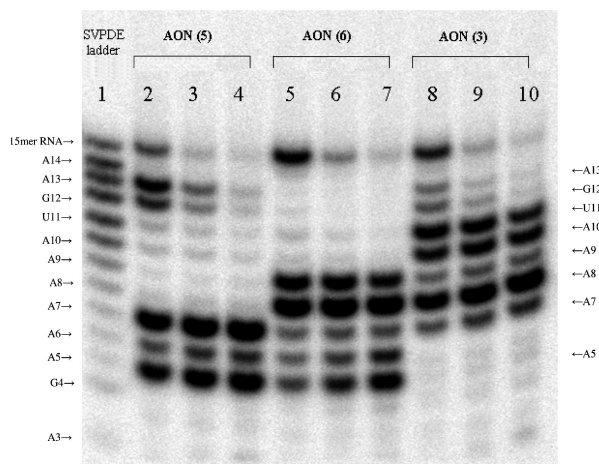
Fig. 4 RNase H hydrolysis of the target RNA (7) when hybridized to the AONs (3), (5) and (6): Lane 1 represents the snake venom phosphodiesterase ladder of the target RNA; Lanes 2, 3 and 4 correspond to the cleavage reaction promoted by the AON (5), after 30, 60 and 120 min, respectively; Lanes 5, 6 and 7 correspond to the cleavage reaction promoted by the AON (6), after 30, 60 and 120 min, respectively; Lanes 8, 9 and 10 correspond to the cleavage reaction promoted by the AON (3), after 30, 60 and 120 min, respectively.
