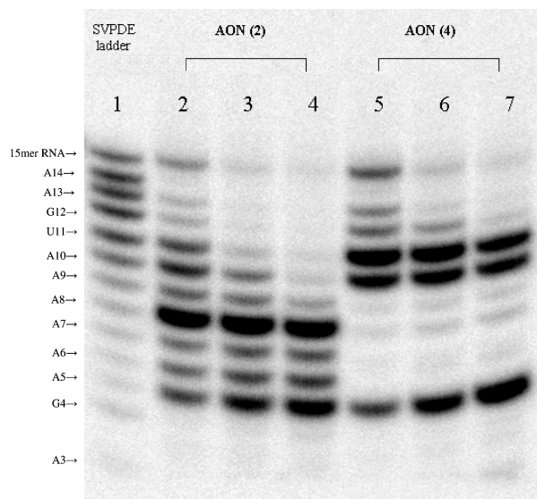
Fig. 3 RNase H hydrolysis of the target RNA (7) when hybridized to the AONs (2) (native) and (4): Lane 1 represents the snake venom phosphodiesterase ladder of the target RNA; Lanes 2, 3 and 4 correspond to the cleavage reaction promoted by the native AON (2), after 30, 60 and 120 min, respectively; Lanes 5, 6 and 7 correspond to the cleavage reaction promoted by the AON (4), after 30, 60 and 120 min, respectively.
