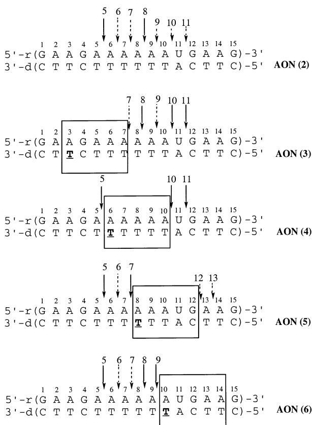
Fig. 5 RNase H cleavage pattern of the hybrid duplexes formed by the AONs (2)–(6) and the RNA target (7). Solid and dashed arrows represent the major and the minor cleavage sites, respectively, at complete degradation (2 h of incubation). Short arrows demonstrate the sites accessible for cleavage at the initial reaction times (30 min of incubation). Boxes represent the parts of the RNA sequence insensitive to RNase H cleavage as the result of the AON modification.
