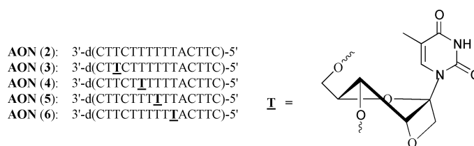
Scheme 1 Reagents and conditions: (i) 4-toluoyl chloride, pyridine, rt, overnight; (ii) silylated base, TMSOTf, acetonitrile, 4 °C, 1 h, rt, 18 h; (iii) MsCl, pyridine, 4 °C, overnight; (iv) 90% aq. \text{CF}_3\text{COOH} , rt, 20 min.; (v) NaH, DMF, 4 °C, 9 h; (vi) methanolic \text{NH}_3 , rt, 2 d; (vii) DMTrCl, pyridine, rt, overnight; (viii) 2-cyanoethyl- N,N -diisopropylchlorophosphoramidite, N,N -diisopropylethylamine, acetonitrile, rt, 2 h.
