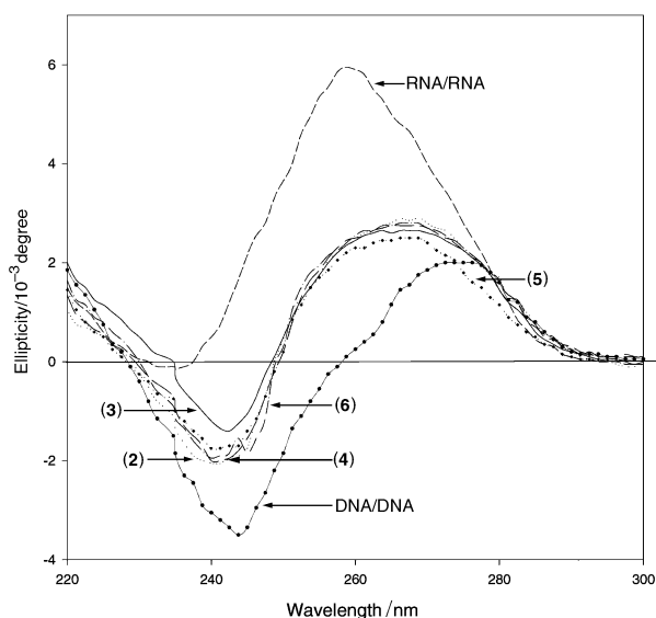
Fig. 2 CD spectra of the duplexes formed by the AONs (2)–(6) and the RNA target (7). For comparison, typical B-type and A-type spectra are presented: DNA/DNA duplex formed by AON (2) and complementary DNA: 5'-d(GAAGAAAAAATGAA)-3', and RNA/RNA duplex formed by self-complementary 17mer RNA: 5'-r(UAACAU-GUUUGGACUCU)-3'.
