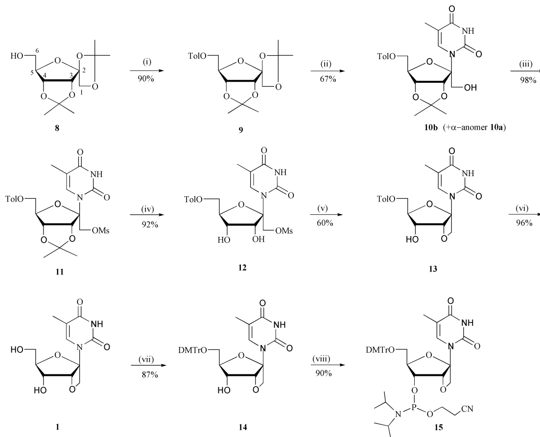
Scheme 1 Reagents and conditions: (i) 4-toluoyl chloride, pyridine, rt, overnight; (ii) silylated base, TMSOTf, acetonitrile, 4 °C, 1 h, rt, 18 h; (iii) MsCl, pyridine, 4 °C, overnight; (iv) 90% aq. \text{CF}_3\text{COOH} , rt, 20 min.; (v) NaH, DMF, 4 °C, 9 h; (vi) methanolic \text{NH}_3 , rt, 2 d; (vii) DMTrCl, pyridine, rt, overnight; (viii) 2-cyanoethyl- N,N -diisopropylchlorophosphoramidite, N,N -diisopropylethylamine, acetonitrile, rt, 2 h.
